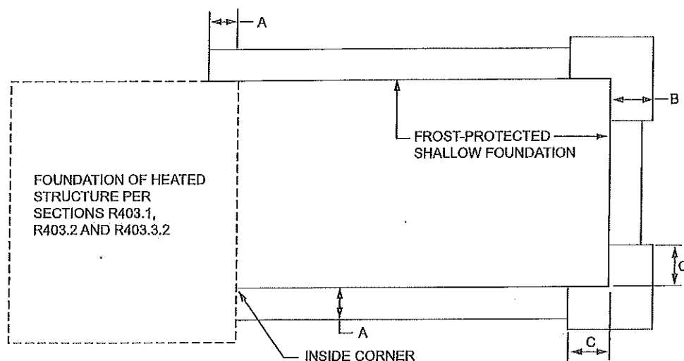
FIGURE R403.3(4)
