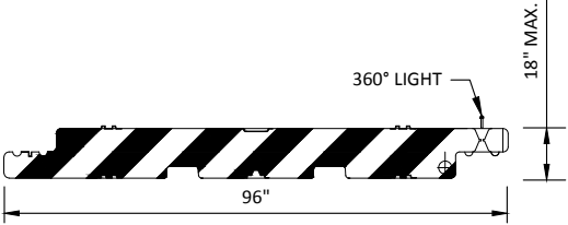
A 3 LOW PROFILE AIRPORT BARRICADE NOT TO SCALE
