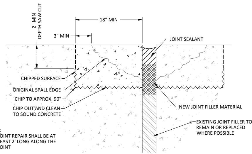
C 6 PARTIAL DEPTH REPAIR - DOUBLE JOINT FACE NOT TO SCALE
