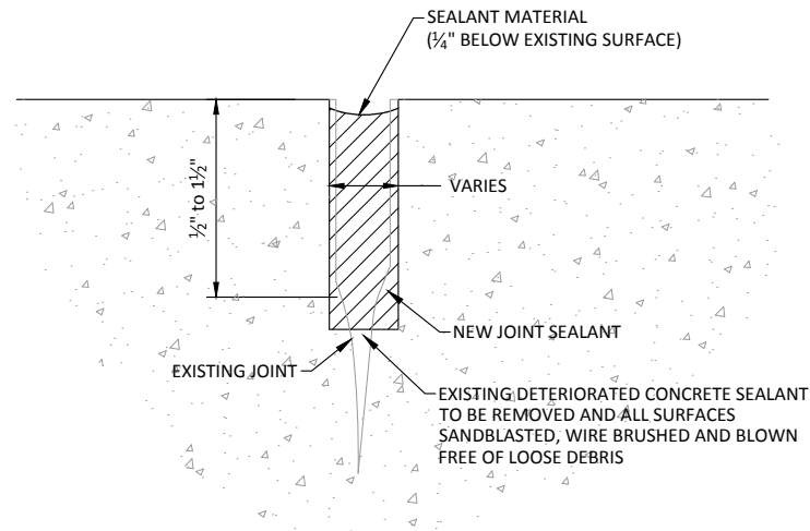
B 6 EXISTING JOINT ROUTE & SEAL NOT TO SCALE
